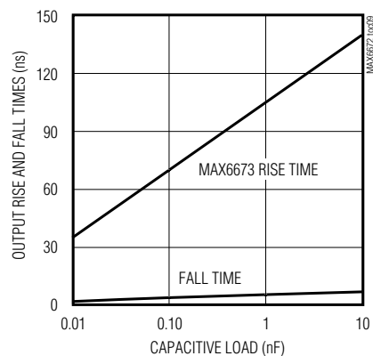
OUTPUT RISE AND FALL TIMES vs. CAPACITIVE LOAD
