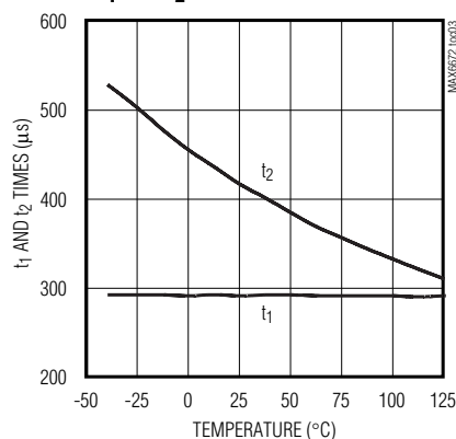
t 1 AND t 2 TIMES vs. TEMPERATURE
