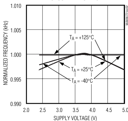
NORMALIZED OUTPUT FREQUENCY vs. SUPPLY VOLTAGE
