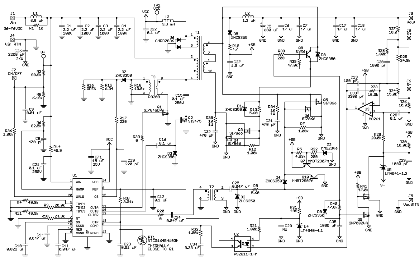
Figure 34. Application Circuit
