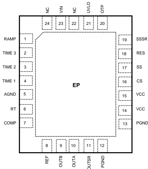
Figure 3. 24-Lead WQFN
