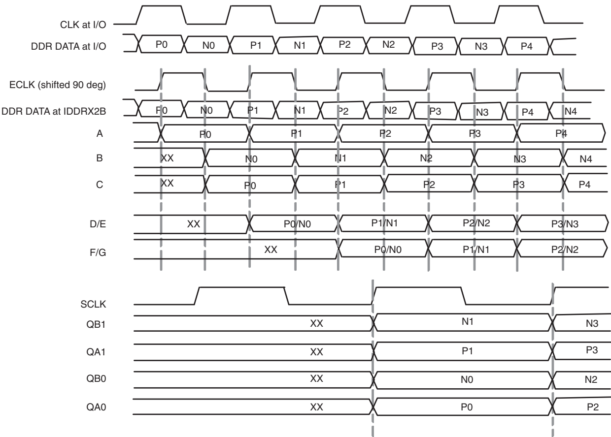
Figure 12-34. IDDRX2B Waveform
