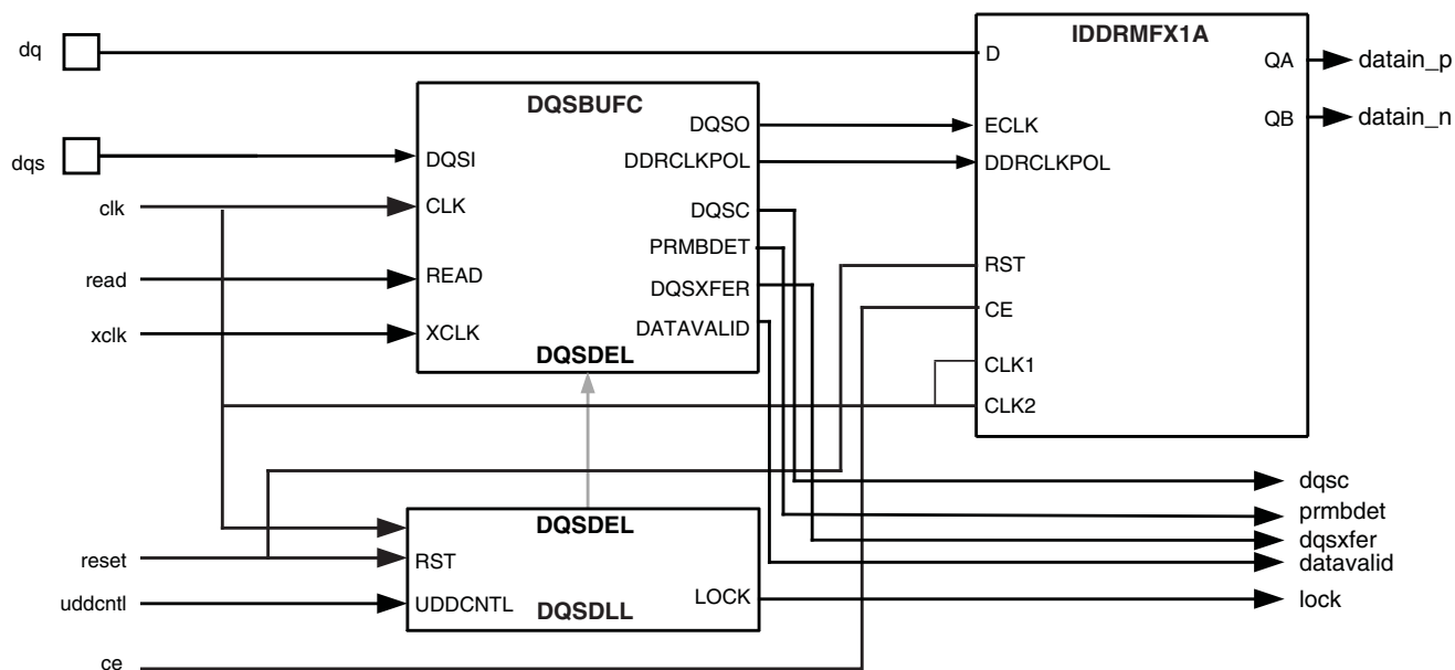
Figure 12-20. Software Primitive Implementation for Memory READ (Full Clock Transfer)
