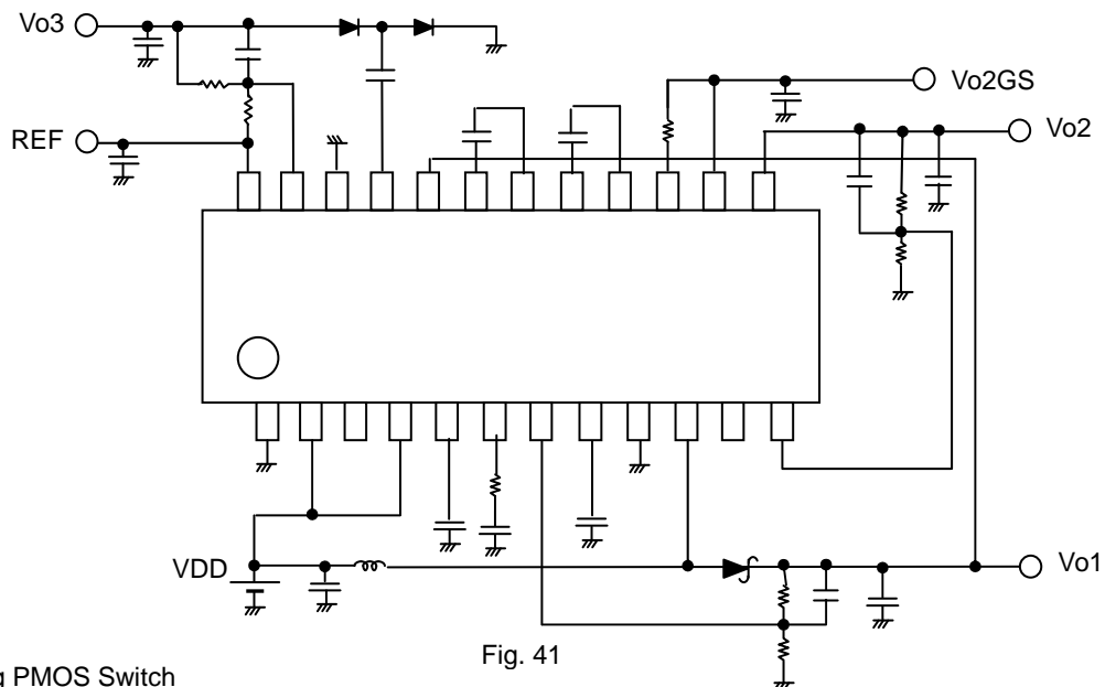
(c) When Inserting PMOS Switch
