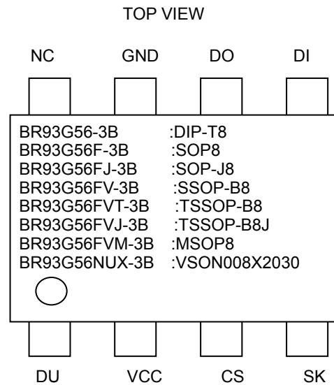
Figure 3. Pin Configuration
