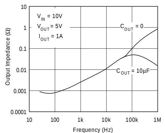
OUTPUT IMPEDANCE
