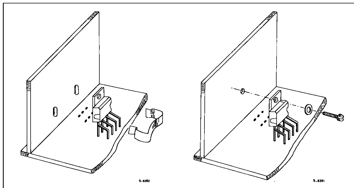
Figure 3 : Mounting Examples
