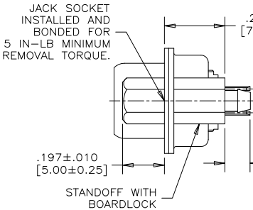
END VIEW
