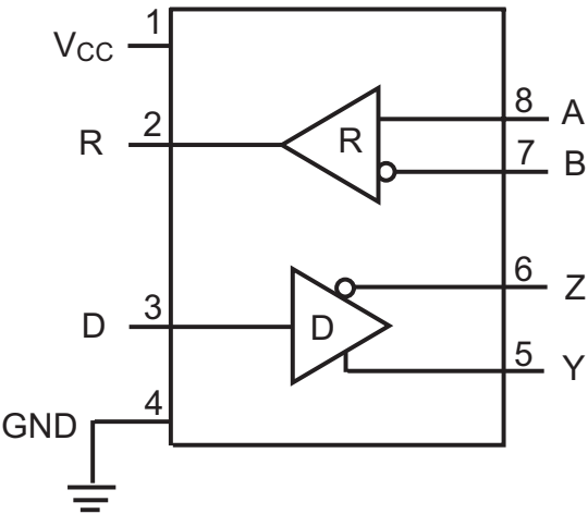
SP490 Pinout (Top View)
