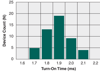
Typical Turn-On Time (N=50, I F =10mA, I L =120mA DC )
