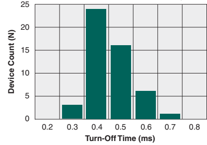
Typical Turn-Off Time (N=50, I F =10mA, I L =120mA DC )
