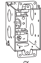
CX Ears flush
