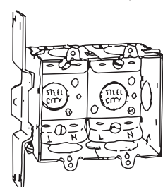
LXWV 2G 2-gang with "CV" bracket recessed 1/8"
