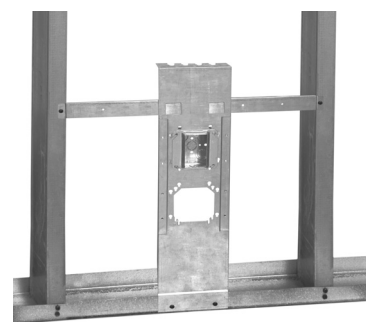
SV1218 mounted to floor track and studs with one 4" square box installed.
