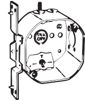
54171NV-25 "V" bracket recessed 1/2"
