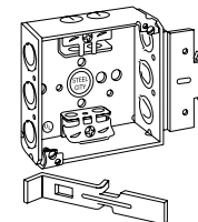
52151 MS X* "MS" bracket for 1½", 2½", 3½", 4" metal studs
