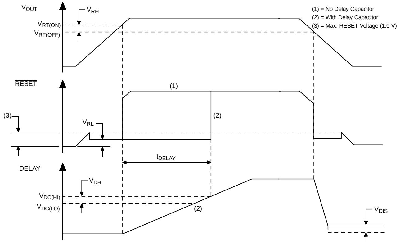
Figure 12. \overline{\text{RESET}} Circuit Waveform
