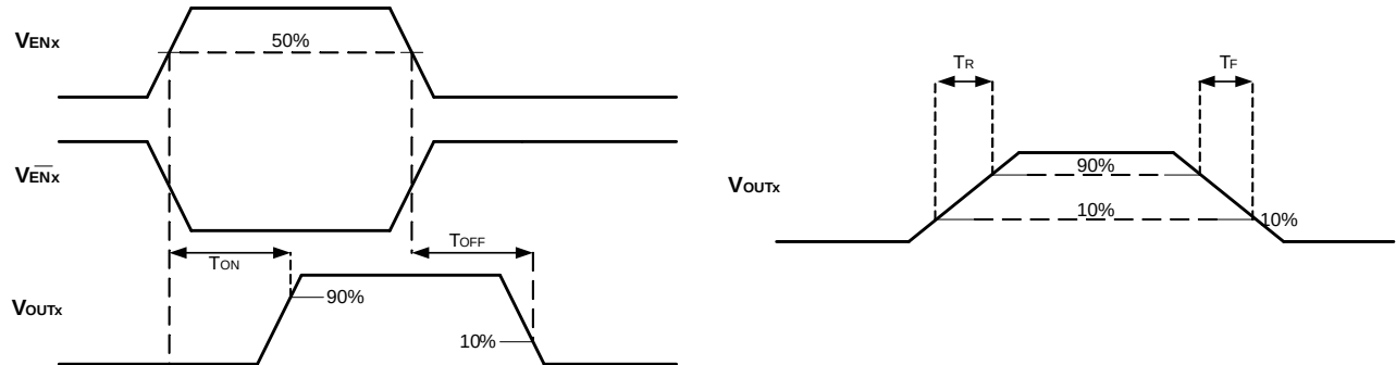
Figure 4. Voltage Waveform
