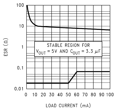
Figure 34. 5V/3.3 \mu F ESR Curves
