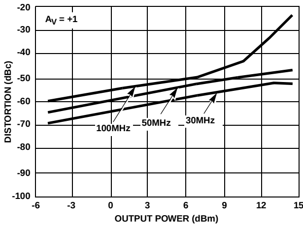
FIGURE 29. SECOND HARMONIC DISTORTION vs P_{\text{OUT}}
