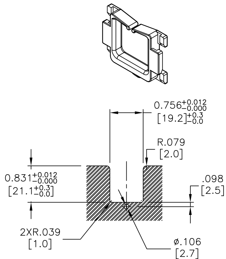
PANEL CUT-OUT DETAIL
