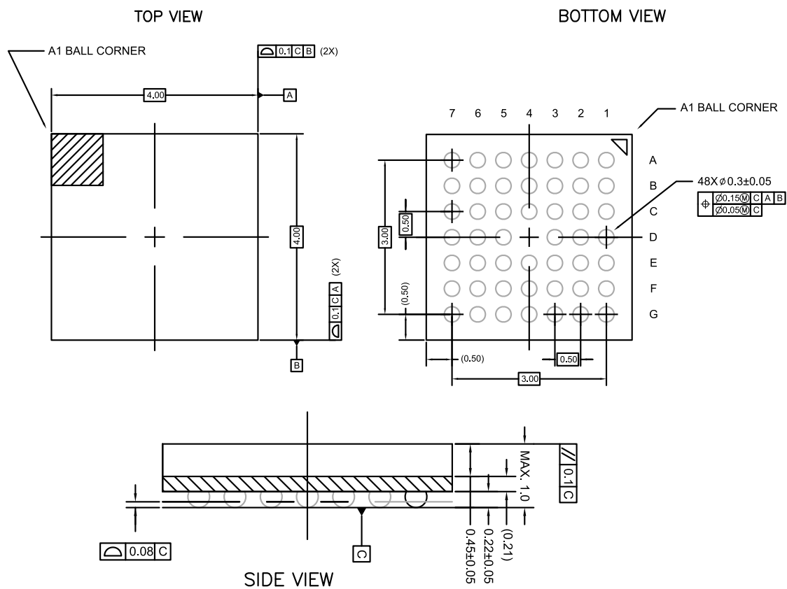
Figure 4.3. BGA48
