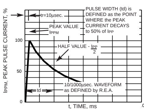
FIG. 3 - PULSE WAVEFORM
