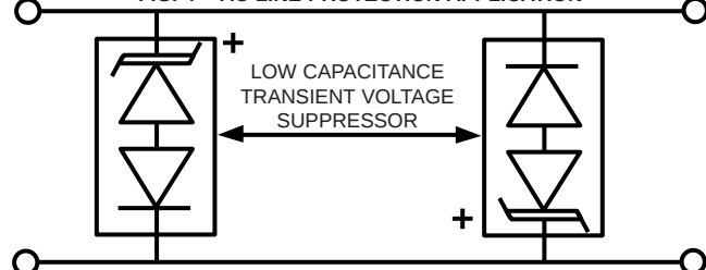
FIG. 4 - AC LINE PROTECTION APPLICATION
