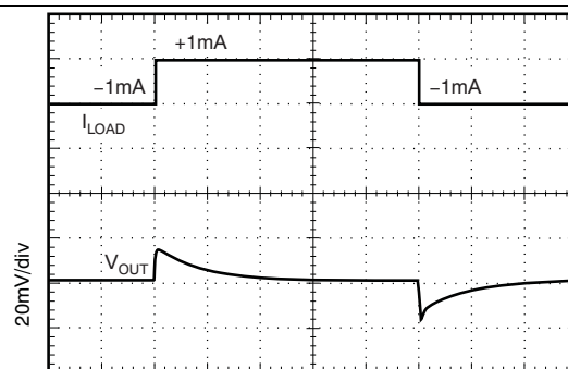
200μs/div C_L = 1\text{ }\mu\text{F} , \pm 1\text{-mA} Output Pulse
