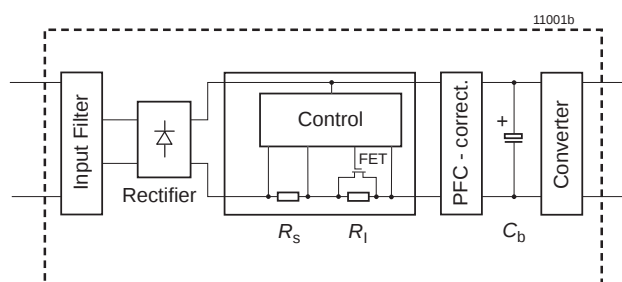
Fig. 33 Option E block diagram
