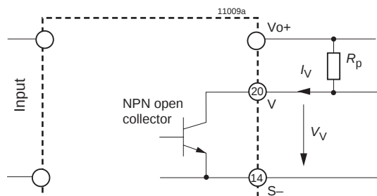
Fig. 42 Output configuration of options V2 and V3
