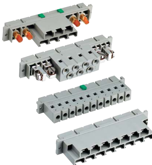
H15, H15S2, and H15S4 female connectors with code key system
