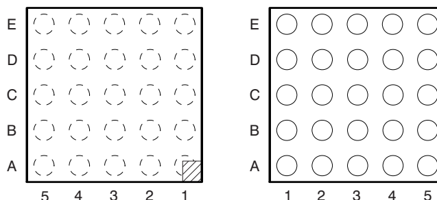
Pin Assignments
