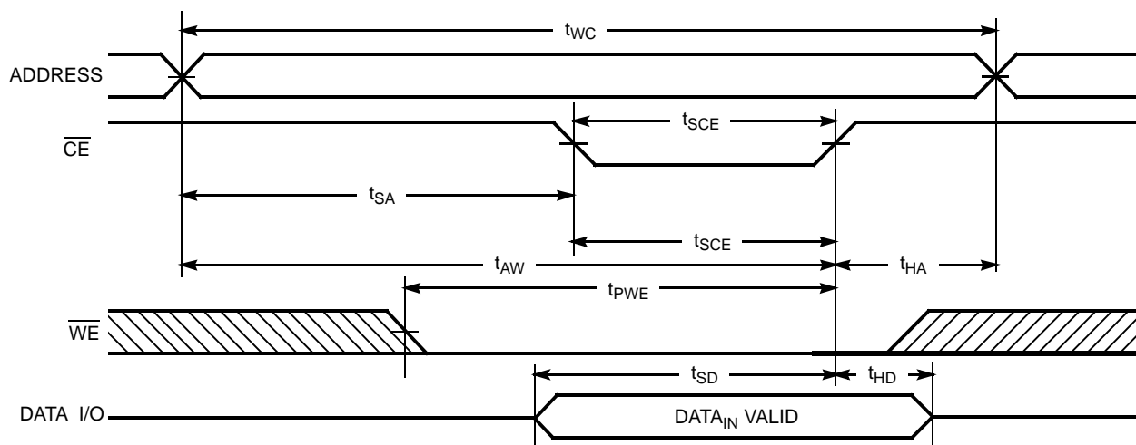
Figure 7. Write Cycle No. 3 ( \overline{\text{CE}} Controlled) [17, 19]
