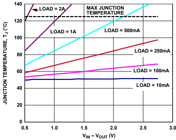
Figure 15. 500 mm 2 of PCB Copper, T_A = 50^\circ\text{C} , LFCSP
