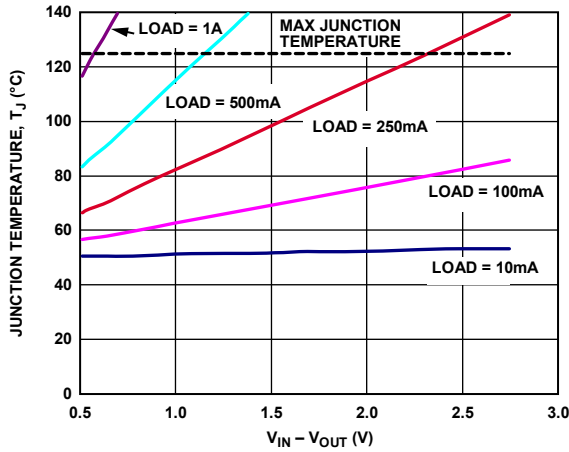
Figure 16. 0 mm 2 of PCB Copper, T_A = 50^\circ\text{C} , LFCSP
