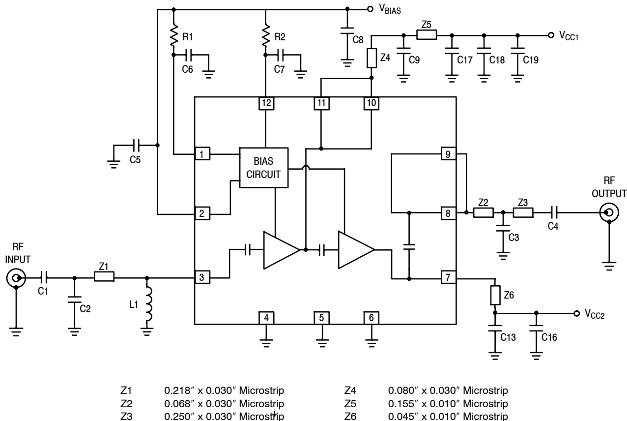
Figure 11. MMA20312BT1 Test Circuit Schematic — W-CDMA
