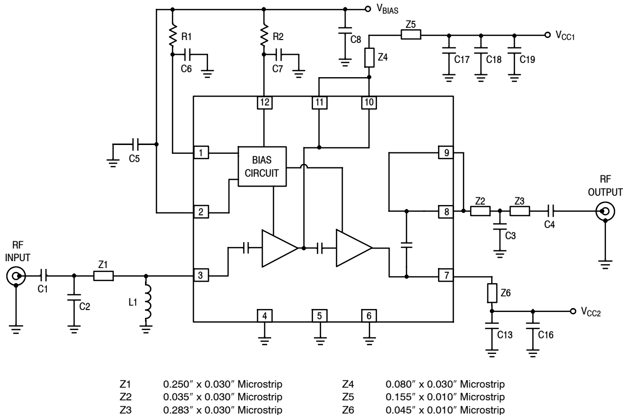
Figure 3. MMA20312BT1 Test Circuit Schematic — TD-SCDMA
