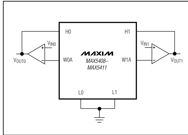
Figure 6. Gain Control
