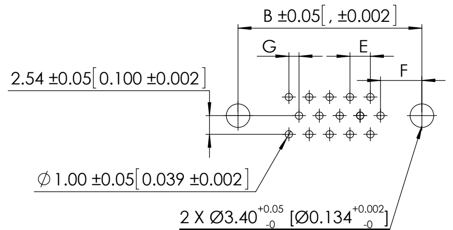
RECOMMENDED PCB LAYOUT 15 POSITIONS FEMALE
