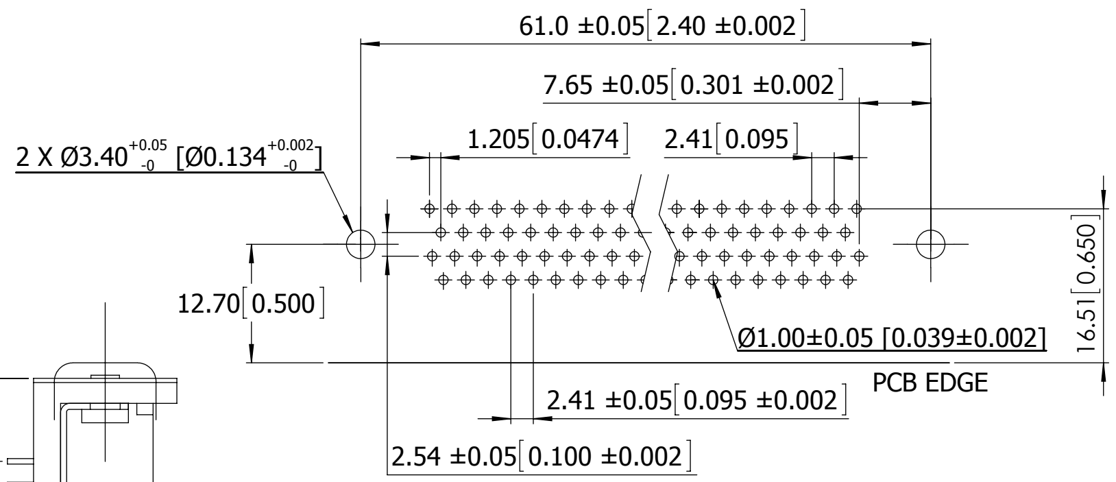
RECOMMENDED PCB LAYOUT 78 POSITIONS MALE / FEMALE
