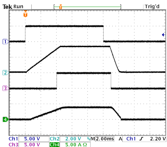
Power Up/Down into 0.825\Omega load: V_{IN}/V_{OUT} = 5V/3.3V , 47nF soft-start capacitor, C_{OUT} \approx 50\mu F Ch.1: ENABLE, Ch. 2: V_{OUT} , Ch. 3: POK, Ch.4: I_{OUT}
