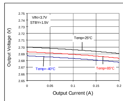
Fig 160. Load Regulation
