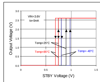
Fig 137. STBY Threshold
