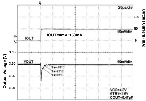
Fig 271. Load Response
