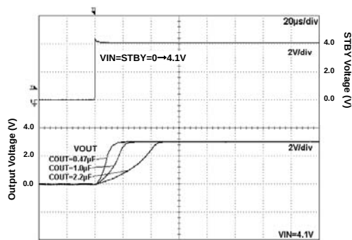
Fig 255. Start Up Time ( V_{IN}=STBY ) I_{out}=0\text{mA}
