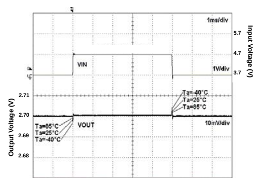
Fig 180. VIN Response
