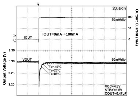
Fig 273. Load Response
