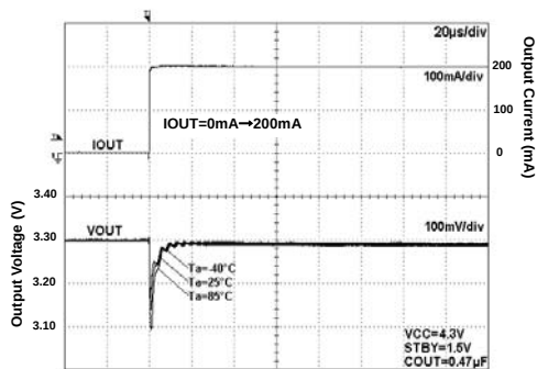
Fig 275. Load Response
