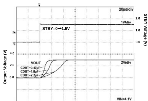
Fig 253. Start Up Time I_{out}=0\text{mA}
