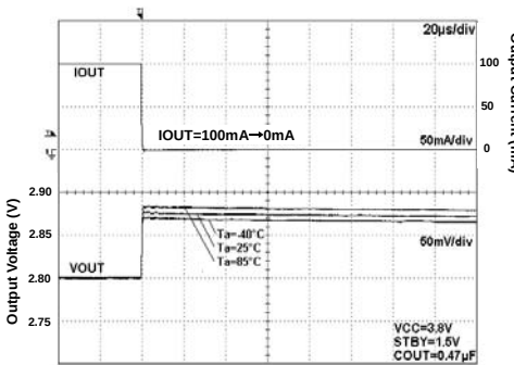
Fig 196. Load Response
