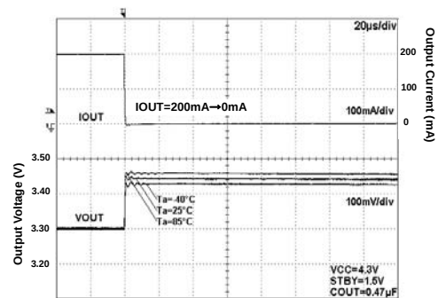
Fig 276. Load Response
