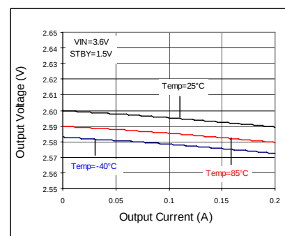
Fig 134. Load Regulation
