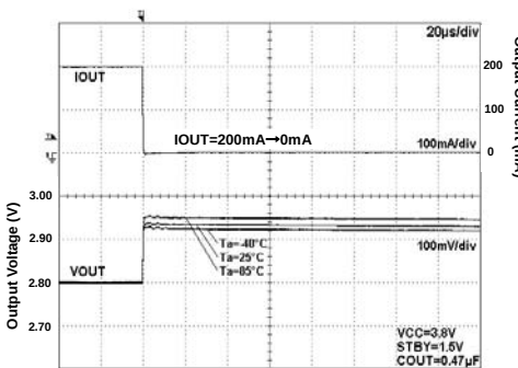
Fig 198. Load Response
