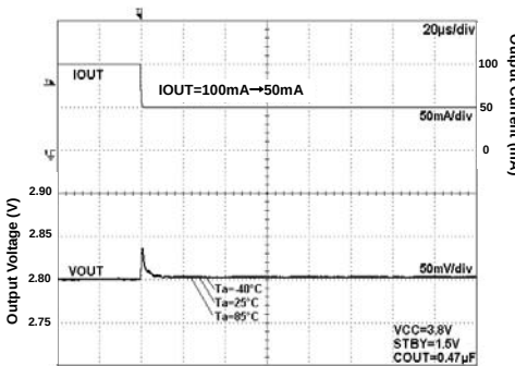
Fig 200. Load Response
