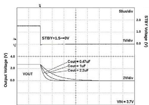
Fig 179. Discharge Time
