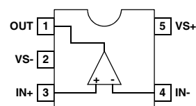
EL5193 (5 LD SOT-23) TOP VIEW
