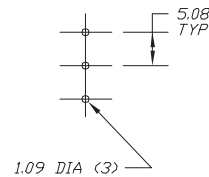
P.C. MOUNTING
