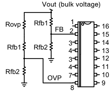
Figure 12. Another Configuration with Two Separate Feed-back Networks
