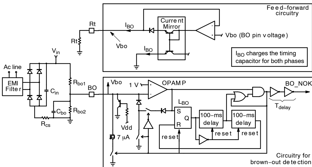
Figure 6. Brown-out Block
