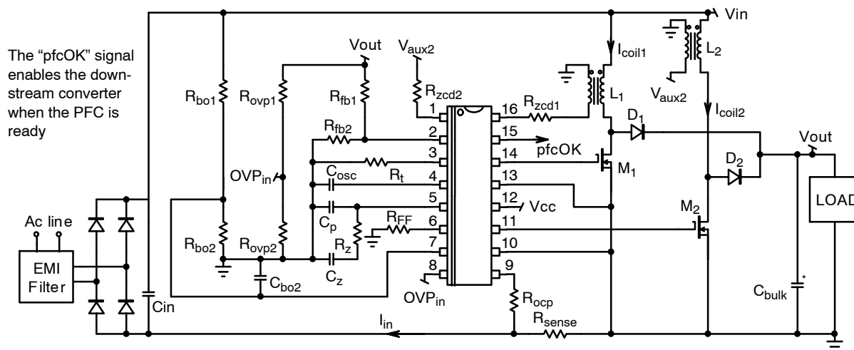
Figure 2. Generic Application Schematic
