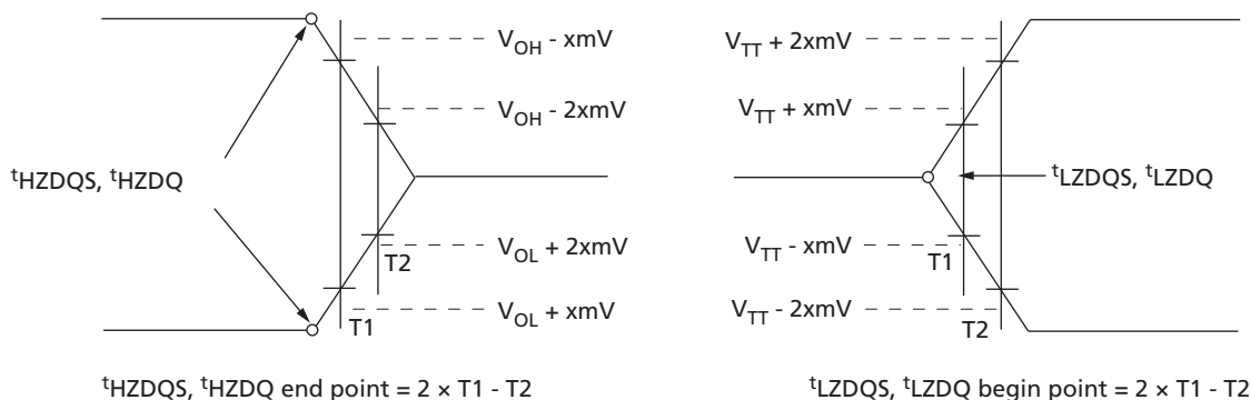
Figure 76: Method for Calculating t_{HZ} and t_{LZ}
