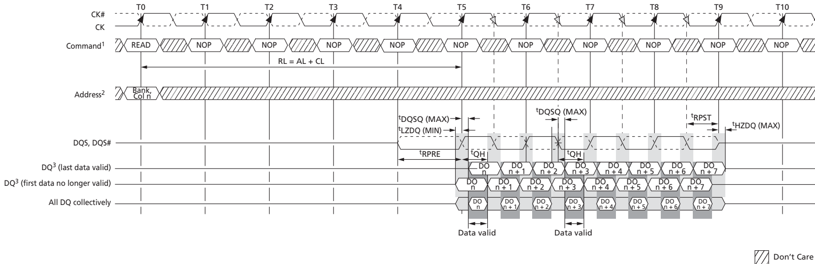
Figure 74: Data Output Timing – t_{DQSQ} and Data Valid Window
