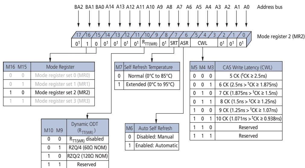
Figure 53: Mode Register 2 (MR2) Definition
