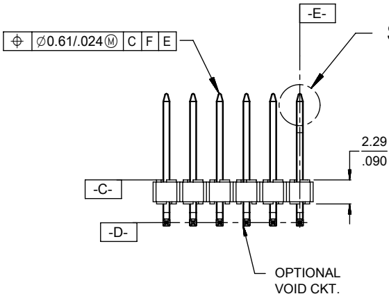
SEE DETAIL Y
