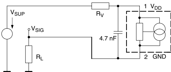
Fig. 5–2: Application Circuit 2
