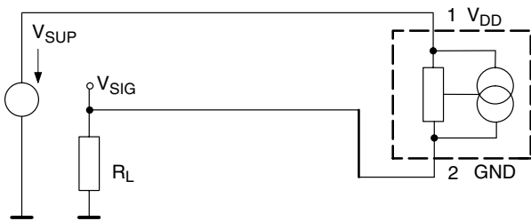
Fig. 5–1: Application Circuit 1
