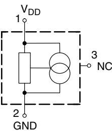
Fig. 1–1: Pin configuration
