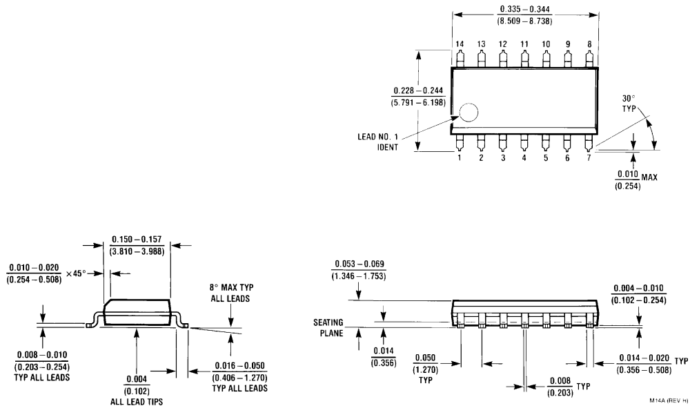
14-Lead Small Outline Molded Package (M) Order Number DM74LS00M NS Package Number M14A
