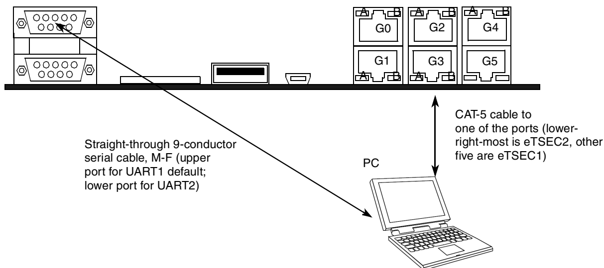
Figure 42. External Connections
