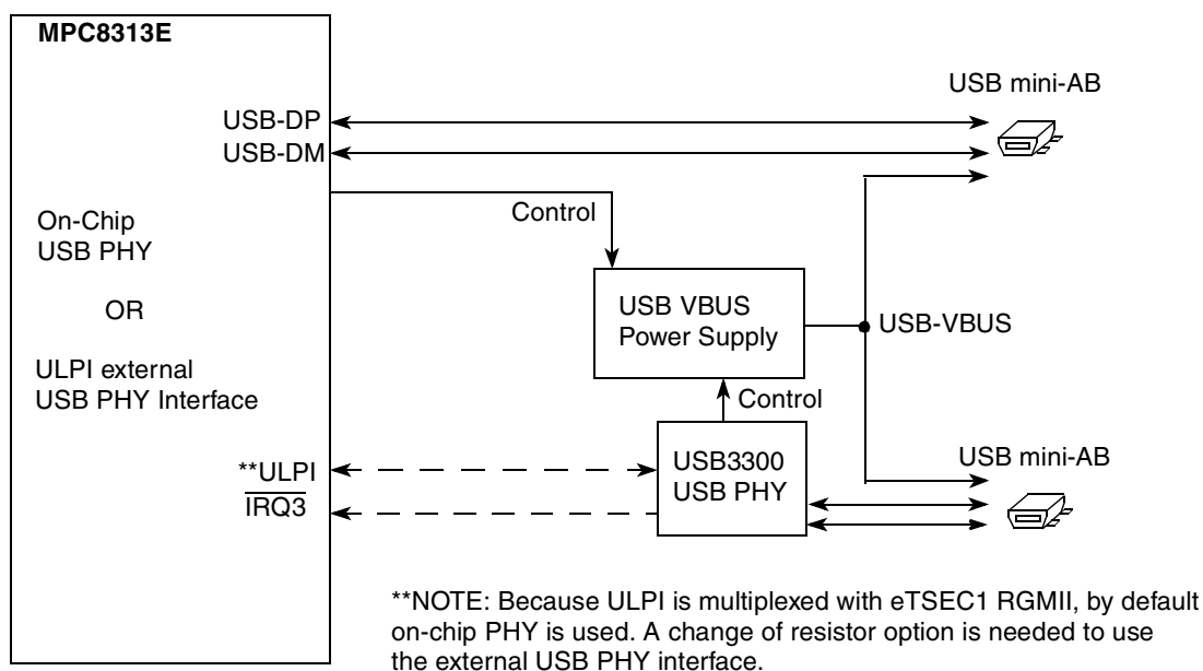
Figure 13. USB Connections
