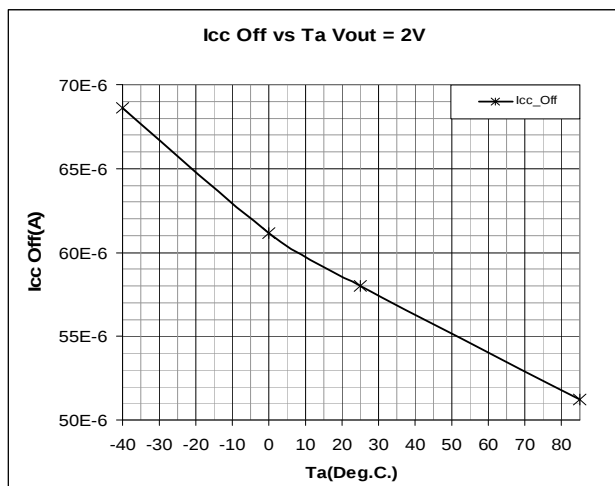
Typical Icc Off vs Ta Vo = 2V
