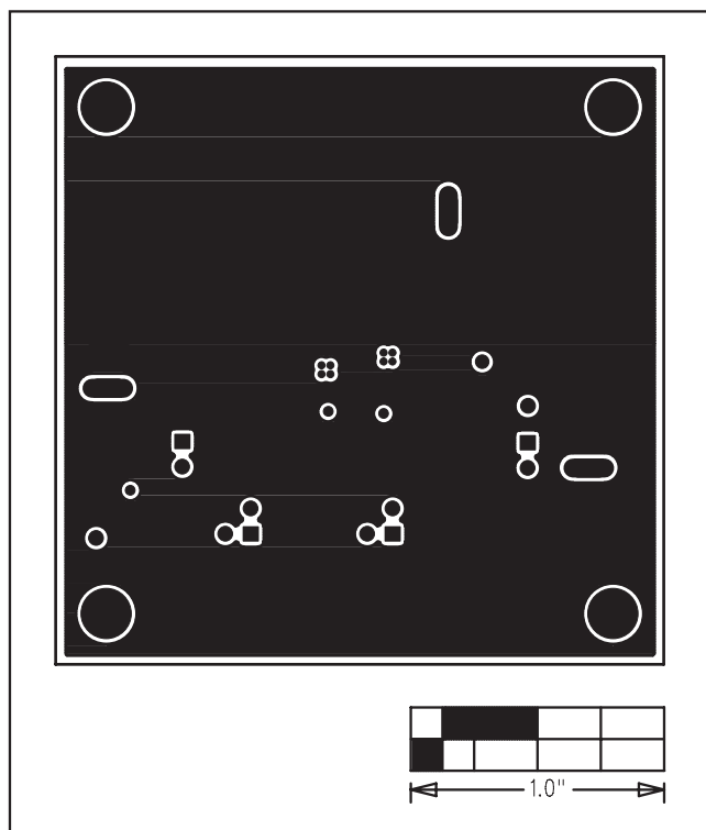
Figure 5. MAX17083 EV Kit PCB Layout—PGND Layer 3
