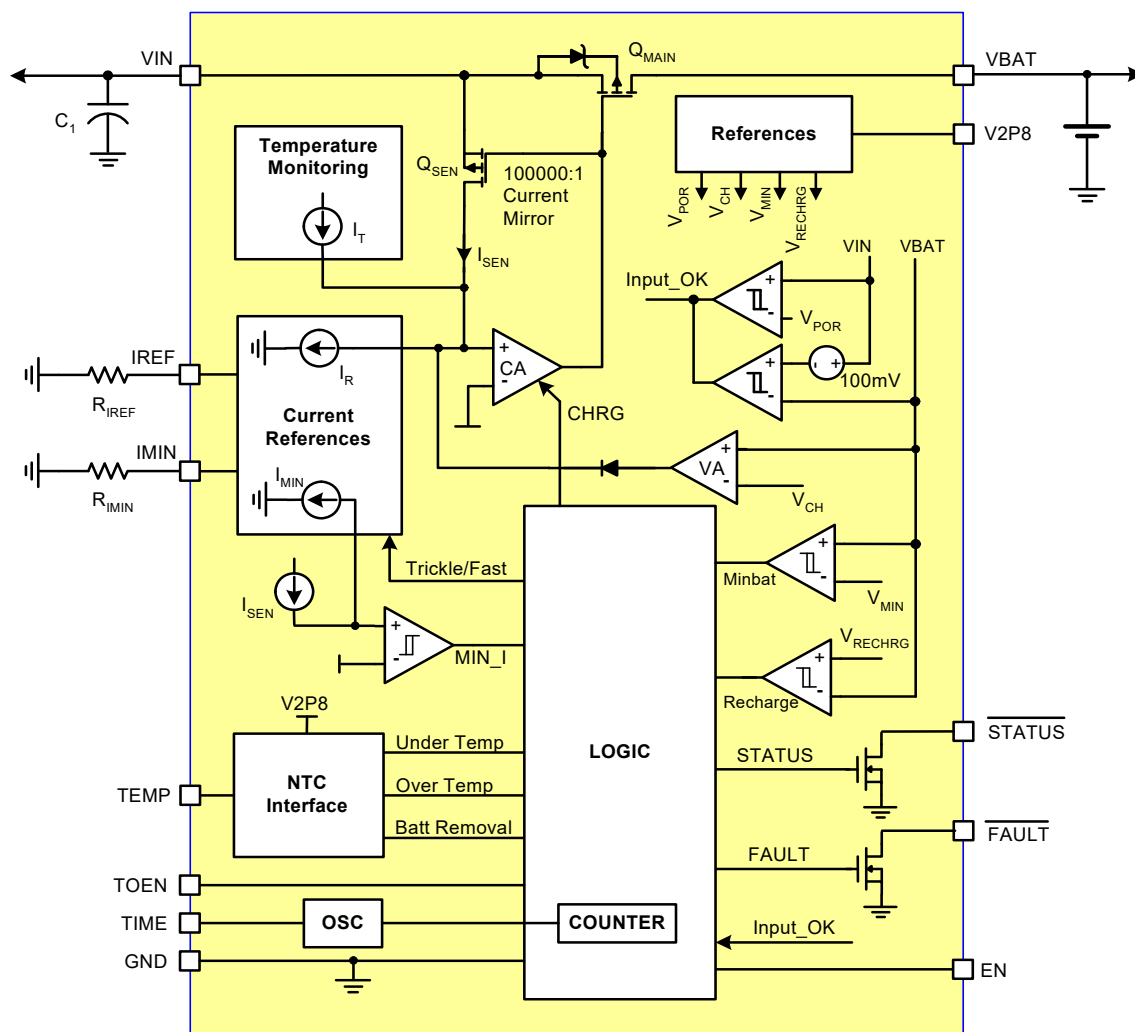
FIGURE 3. BLOCK PROGRAM
