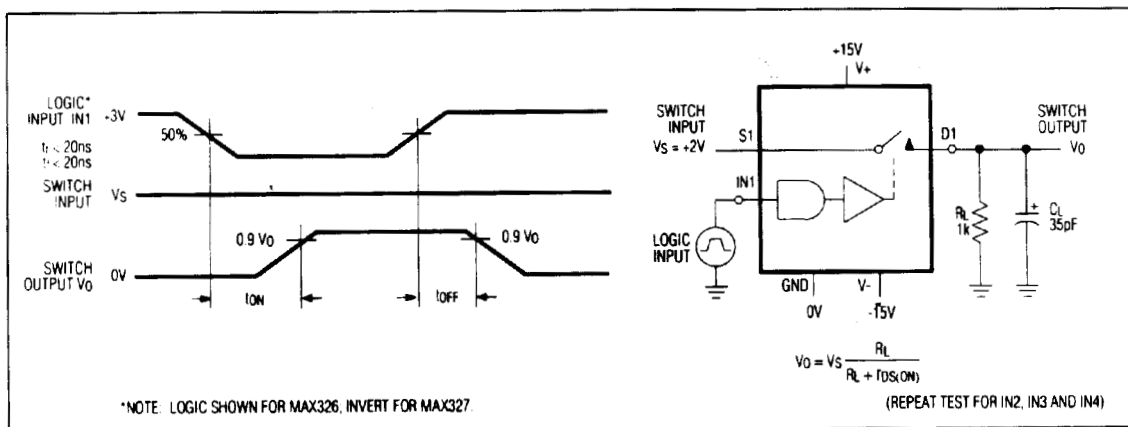
Figure 1. Switching-Time Test Circuit. Switch-output waveform shown for V_S = \text{constant} with logic-input waveform as shown. Note: V_S may be positive or negative as per switching-time test circuit. V_O is the steady-state output with switch on. Feedthrough via gate capacitance may result in spikes at leading and trailing edge of output waveform.
