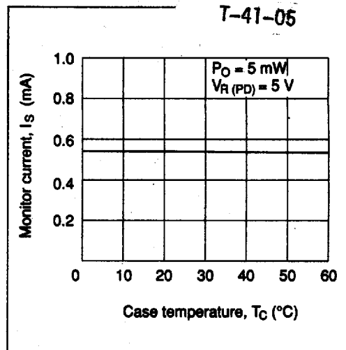
Figure 8 Monitor Current vs. Case Temperature (HL7836MG)
