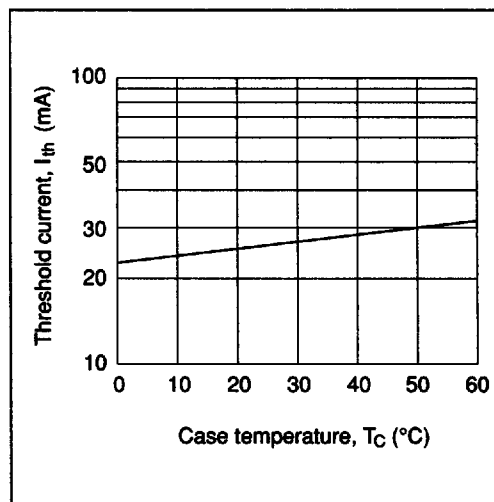
Figure 6 Threshold Current vs. Case Temperature
