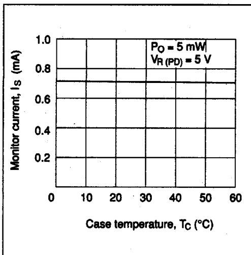
Figure 7 Monitor Current vs. Case Temperature (HL7836G)
