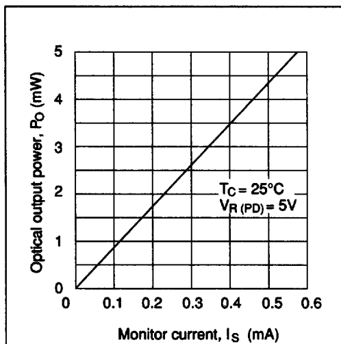
Figure 5 Optical Output Power vs. Monitor Current (HL7836MG)
