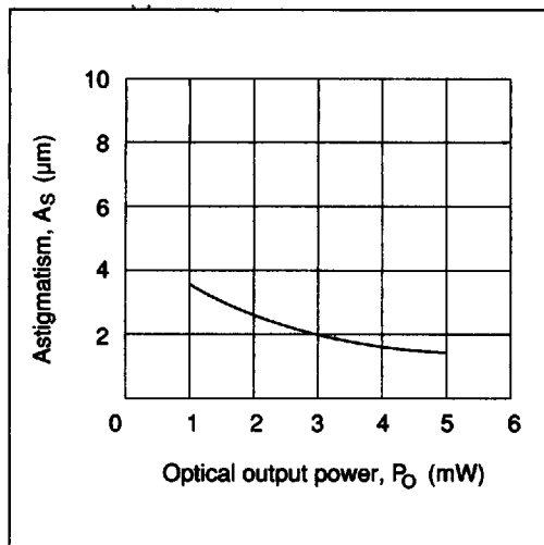
Figure 11 Astigmatism vs. Optical Output Power
