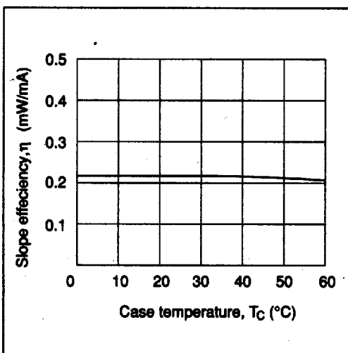
Figure 9 Slope Efficiency vs. Case Temperature
