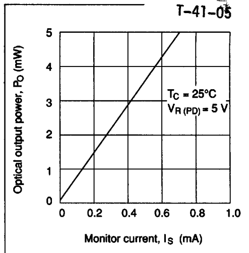
Figure 4 Optical Output Power vs. Monitor Current (HL7836G)
