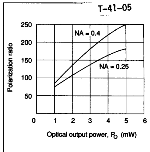
Figure 12 Polarization Ratio vs. Optical Output Power
