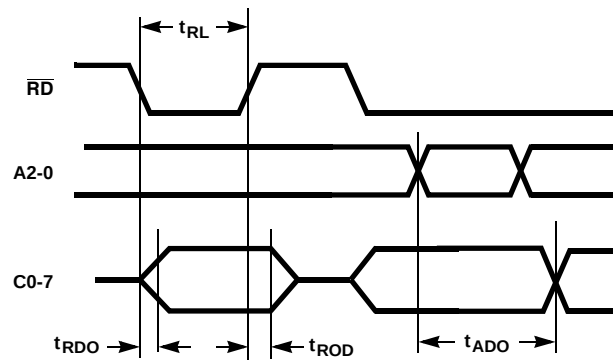
FIGURE 30. TIMING RELATIVE TO READ
