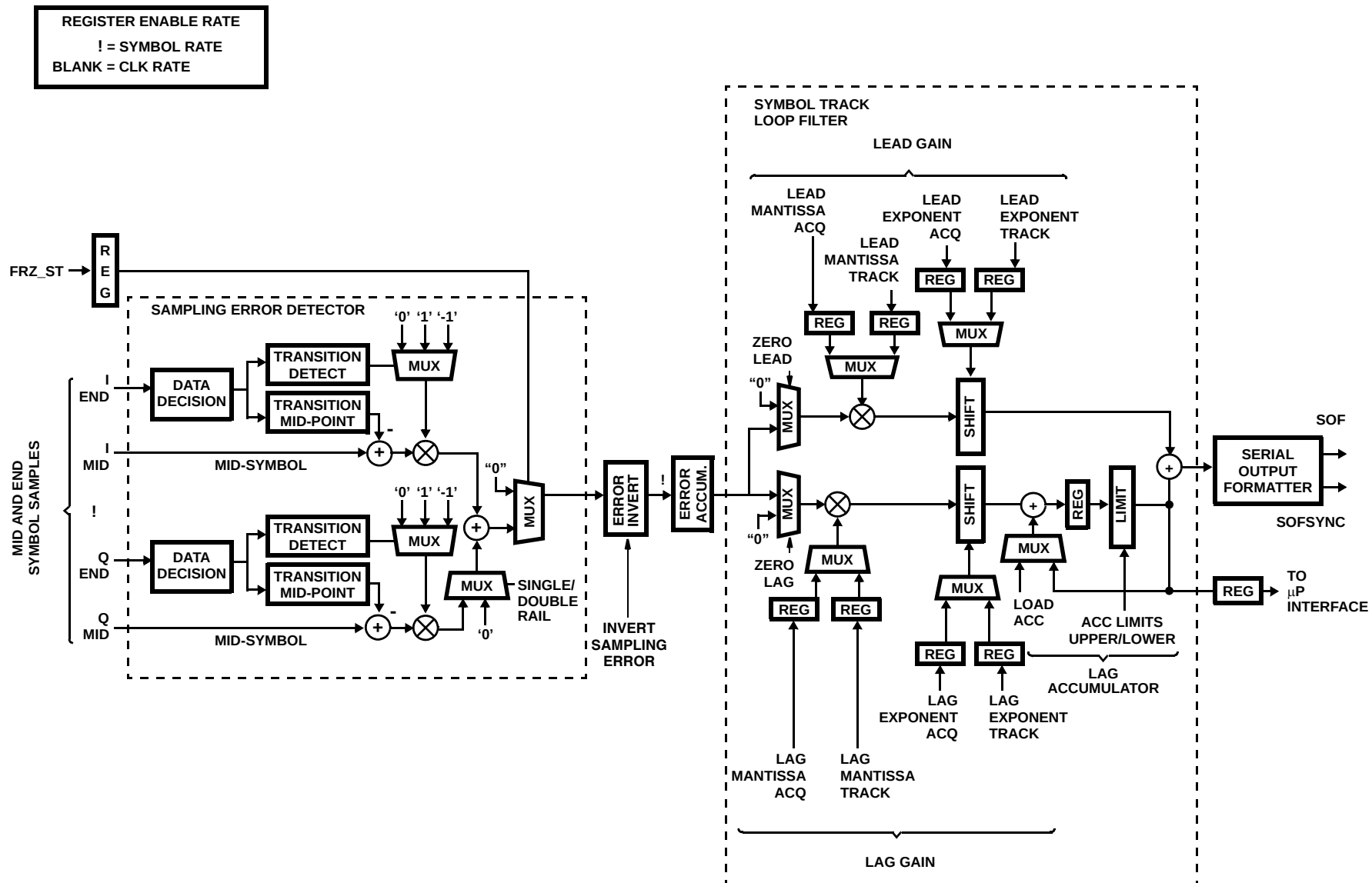
FIGURE 11. SYMBOL TRACKING
