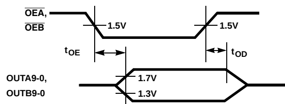
FIGURE 29. OUTPUT ENABLE/DISABLE
