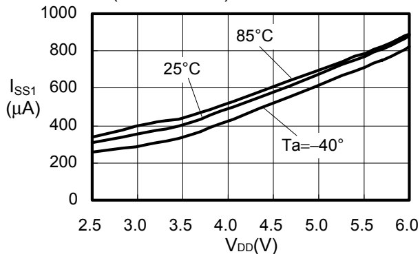
S-8340A33A(fosc:600 kHz)
