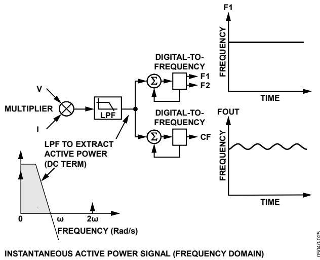
Figure 27. Active Power to Frequency Conversion
