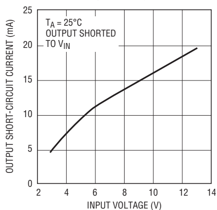
LTC1258-2.5* Output Short-Circuit vs Input Voltage
