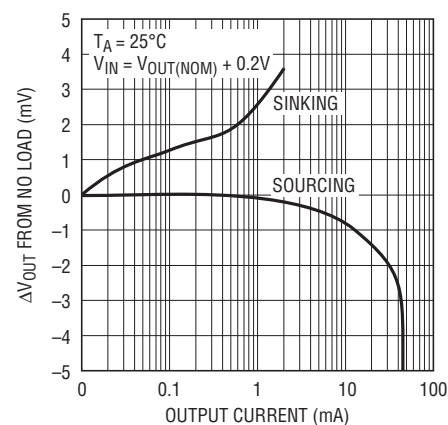
LTC1258 Series Load Regulation
