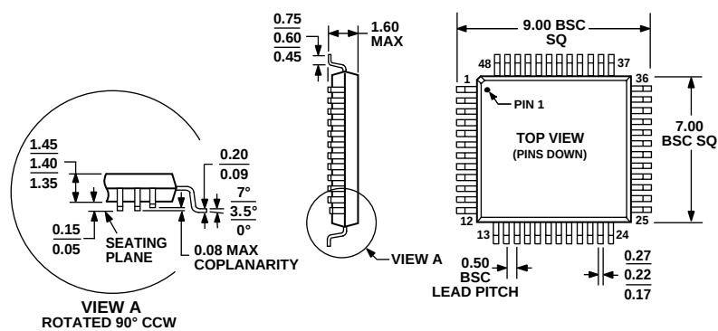
Figure 4. 48-Lead Low Profile Quad Flat Package [LQFP] (ST-48) Dimensions shown in millimeters
