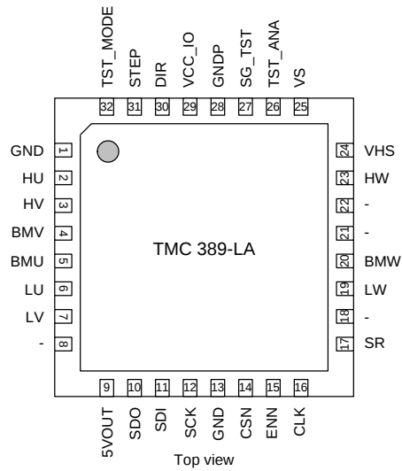
figure 2: TMC389 pinning
