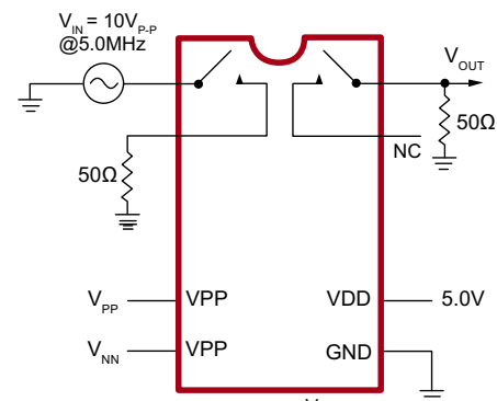
Crosstalk
