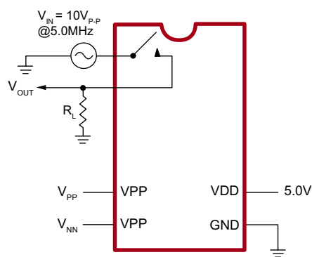
OFF Isolation
