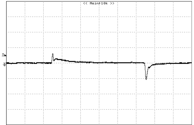
Figure 32: Typical transient response to step load change at 1A/μS from 0%~ 50%~0% of I_o , max at 12Vin, 1.2Vout (Cout = 1uF ceramic, 47uF+10μFceramic) CH1 : VOUT, 0.2V/div, 100uS/div
