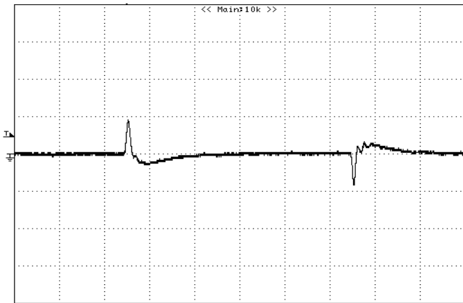
Figure 35: Typical transient response to step load change at 1A/μS from 0%~ 50%~0% of I_o , max at 12Vin, 3.3Vout (Cout = 1uF ceramic, 47uF+10μFceramic) CH1 : VOUT, 0.2V/div, 100uS/div
