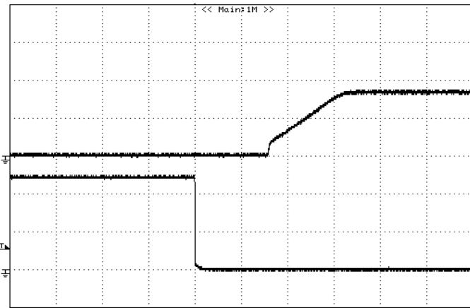
Figure 23: Turn on delay time at remote on 12Vin, 3.3V/12A out. (Top: VOUT, 2V/div; Bottom: ON/OFF, 2V/div; 2mS/div)
