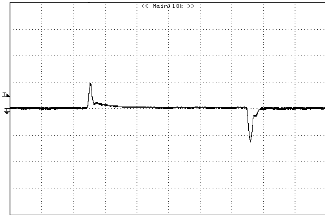
Figure 31: Typical transient response to step load change at 1A/μS from 0%~ 50%~0% of I_o , max at 7Vin, 0.69Vout (Cout = 1uF ceramic, 47uF+10μFceramic) CH1 : VOUT, 0.2V/div, 100uS/div
