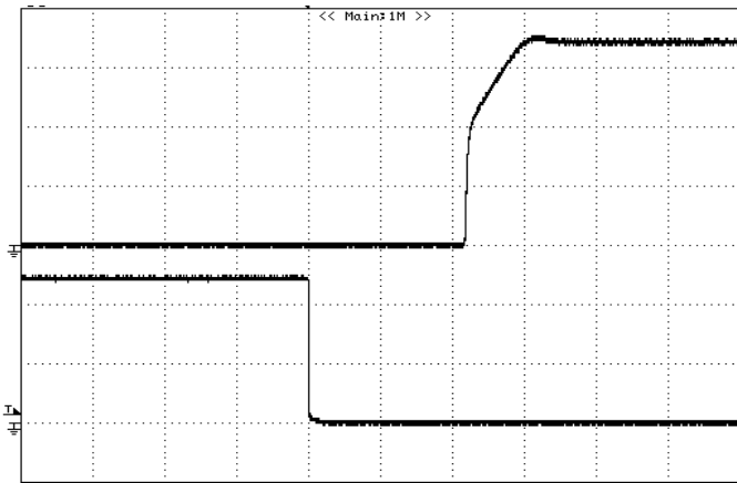
Figure 19: Turn on delay time at remote on 7Vin, 0.69V/12A out. (Top: VOUT, 0.2V/div; Bottom: ON/OFF, 2V/div; 2mS/div)
