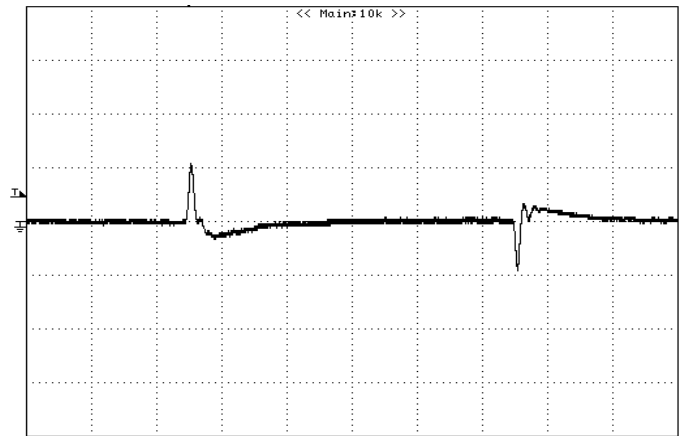
Figure 36: Typical transient response to step load change at 1A/μS from 0%~ 50%~0% of I_o , max at 12Vin, 5.0Vout (Cout = 1uF ceramic, 47uF+10μFceramic) CH1 : VOUT, 0.2V/div, 100uS/div
