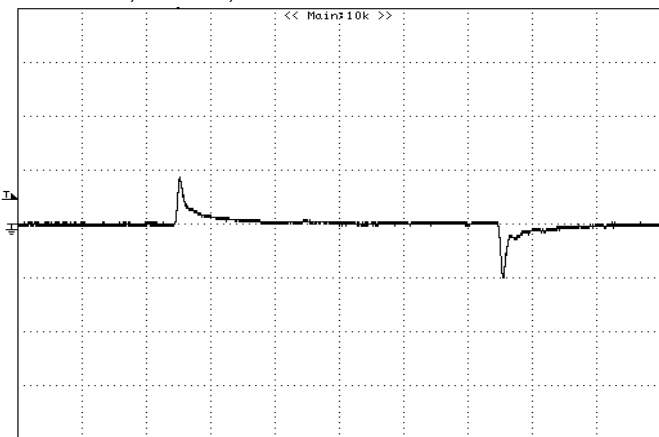
Figure 33: Typical transient response to step load change at 1A/μS from 0%~ 50%~0% of I_o , max at 12Vin, 1.8Vout (Cout = 1uF ceramic, 47uF+10μFceramic) CH1 : VOUT, 0.2V/div, 100uS/div
