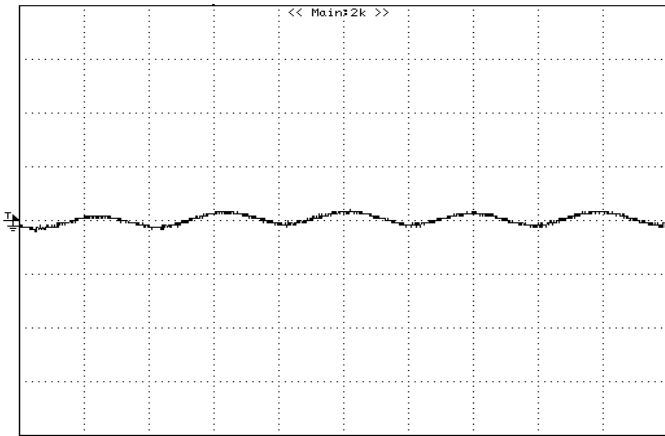
Figure 7: Output ripple & noise at 7Vin, 0.69V/12A out CH1:VOUT, 20mV/div, 1uS/div
