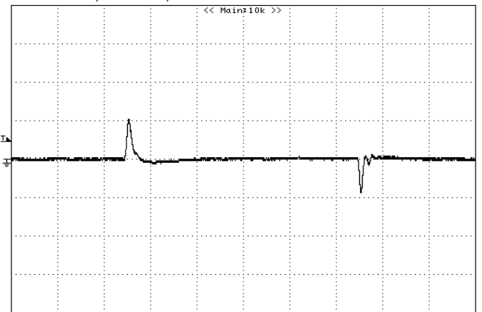
Figure 34: Typical transient response to step load change at 1A/μS from 0%~ 50%~0% of I_o , max at 12Vin, 2.5Vout (Cout = 1uF ceramic, 47uF+10μFceramic) CH1: VOUT, 0.2V/div, 100uS/div
