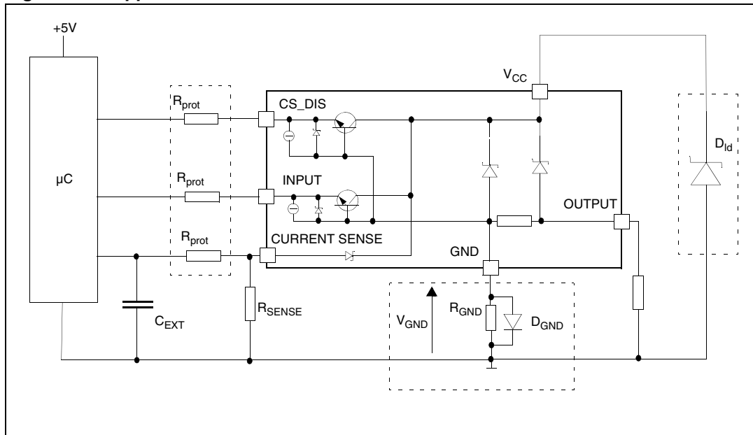
Figure 26. Application schematic (1)
